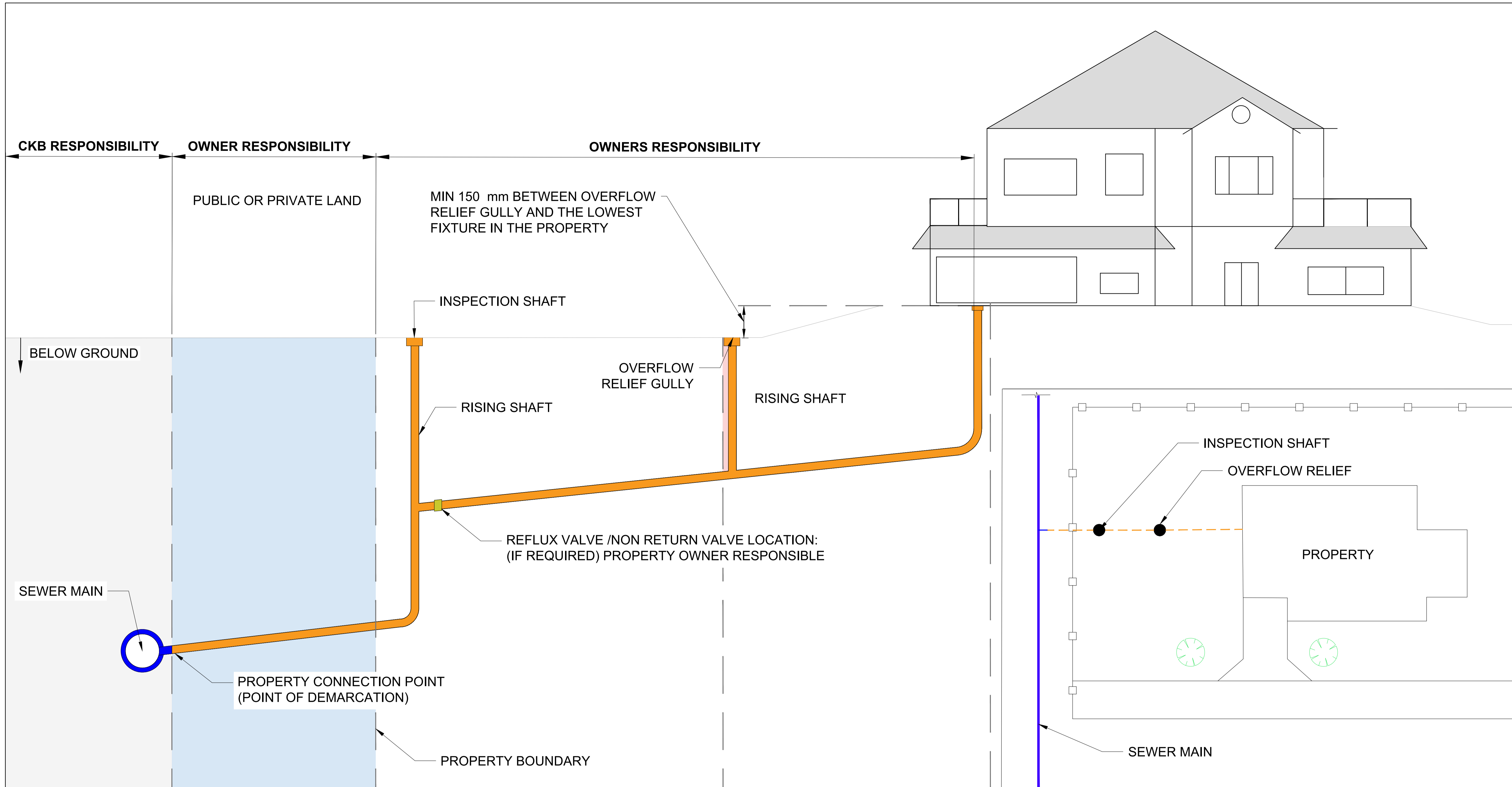
SEWER NETWORK OWNERSHIP - SECTION VIEW SCALE - N.T.S.
